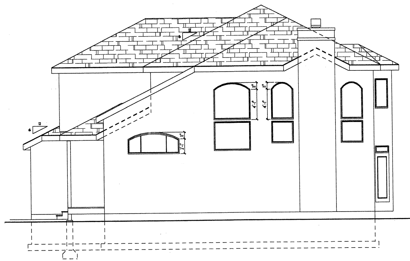
RIGHT ELEVATION 1/8" SCALE
