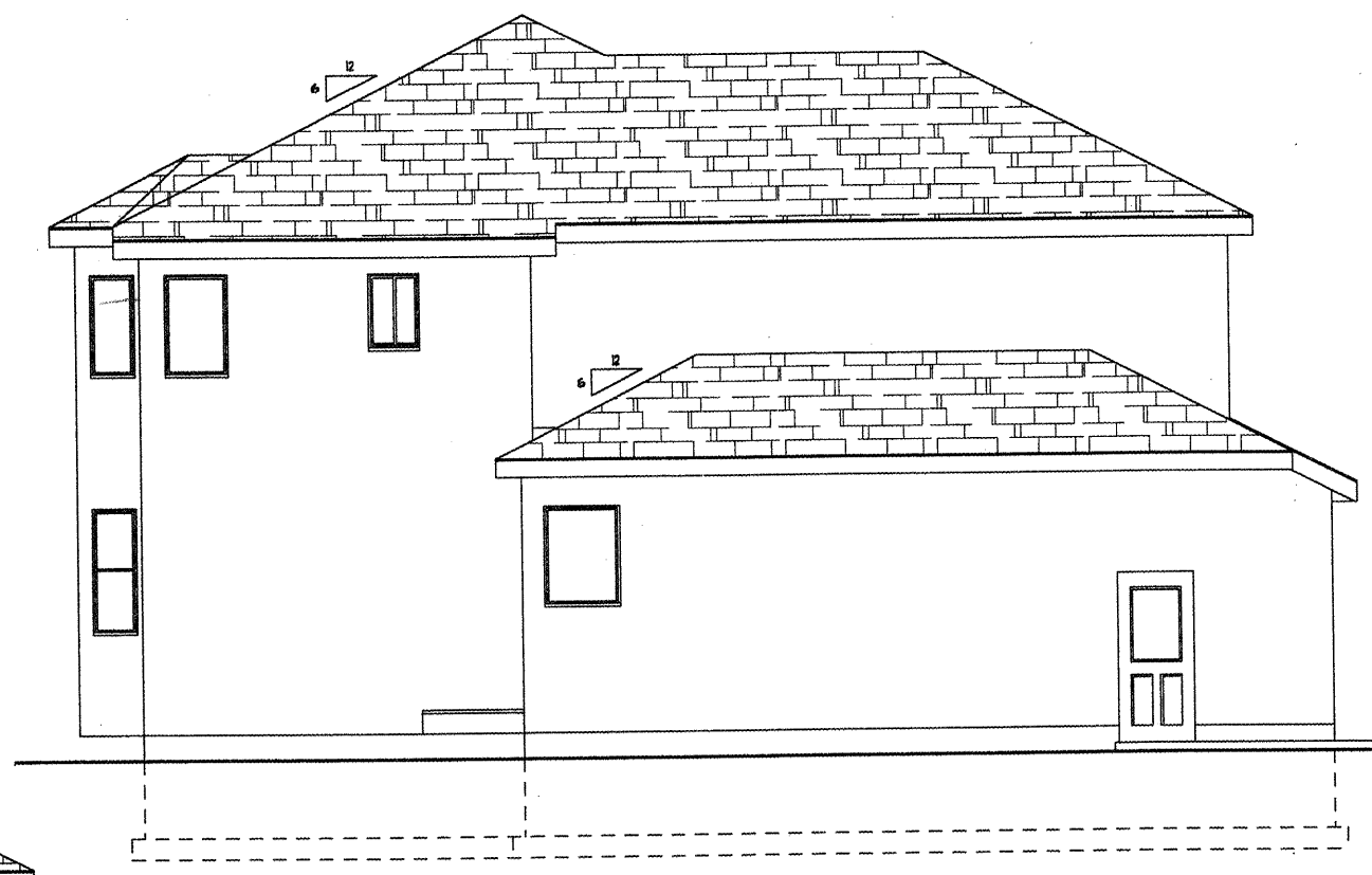
LEFT ELEVATION 1/8" SCALE
